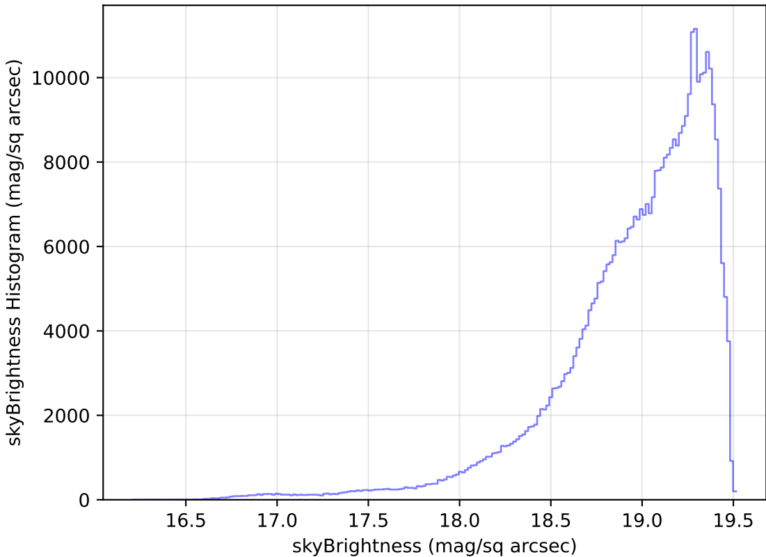
baseline_v3.2_10yrs All sky z band: skyBrightness Histogram
