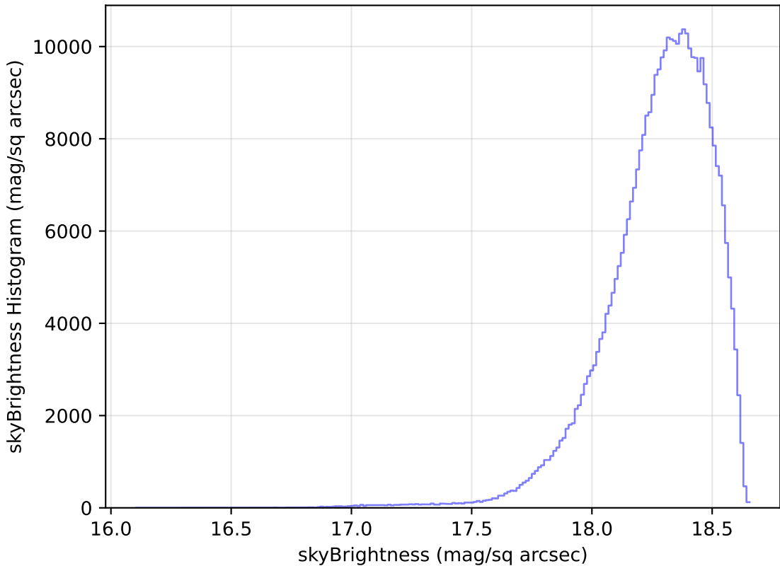
baseline_v3.2_10yrs All sky y band: skyBrightness Histogram
