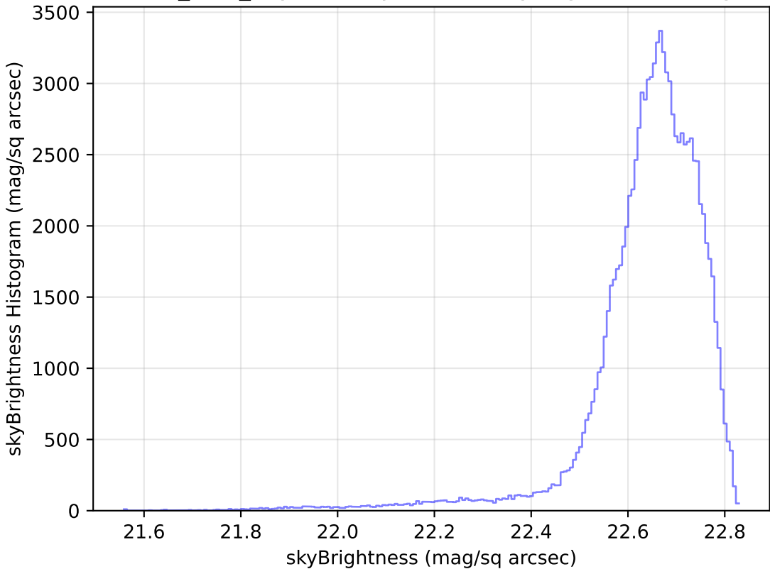
baseline_v3.2_10yrs All sky u band: skyBrightness Histogram
