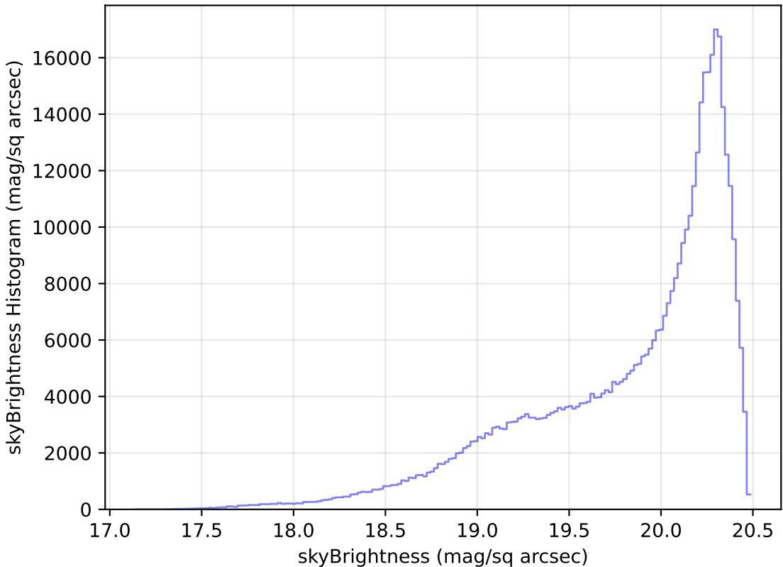
baseline_v3.2_10yrs All sky i band: skyBrightness Histogram
