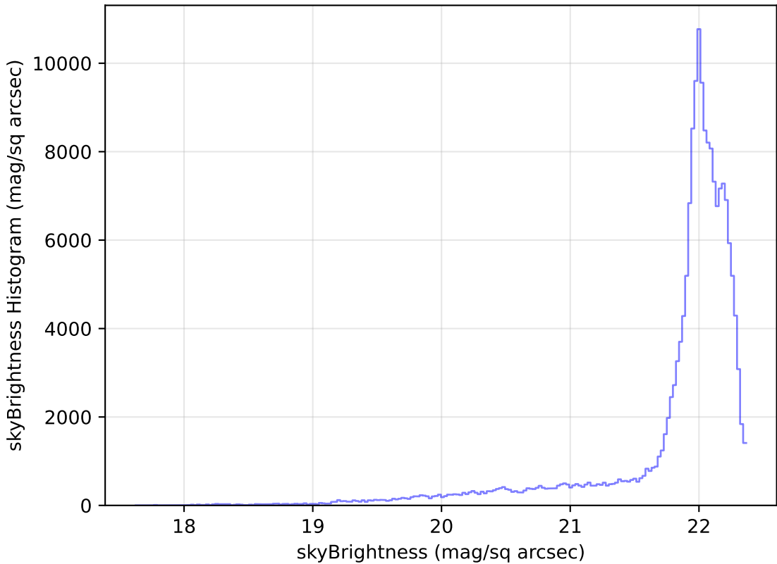
baseline_v3.2_10yrs All sky g band: skyBrightness Histogram
