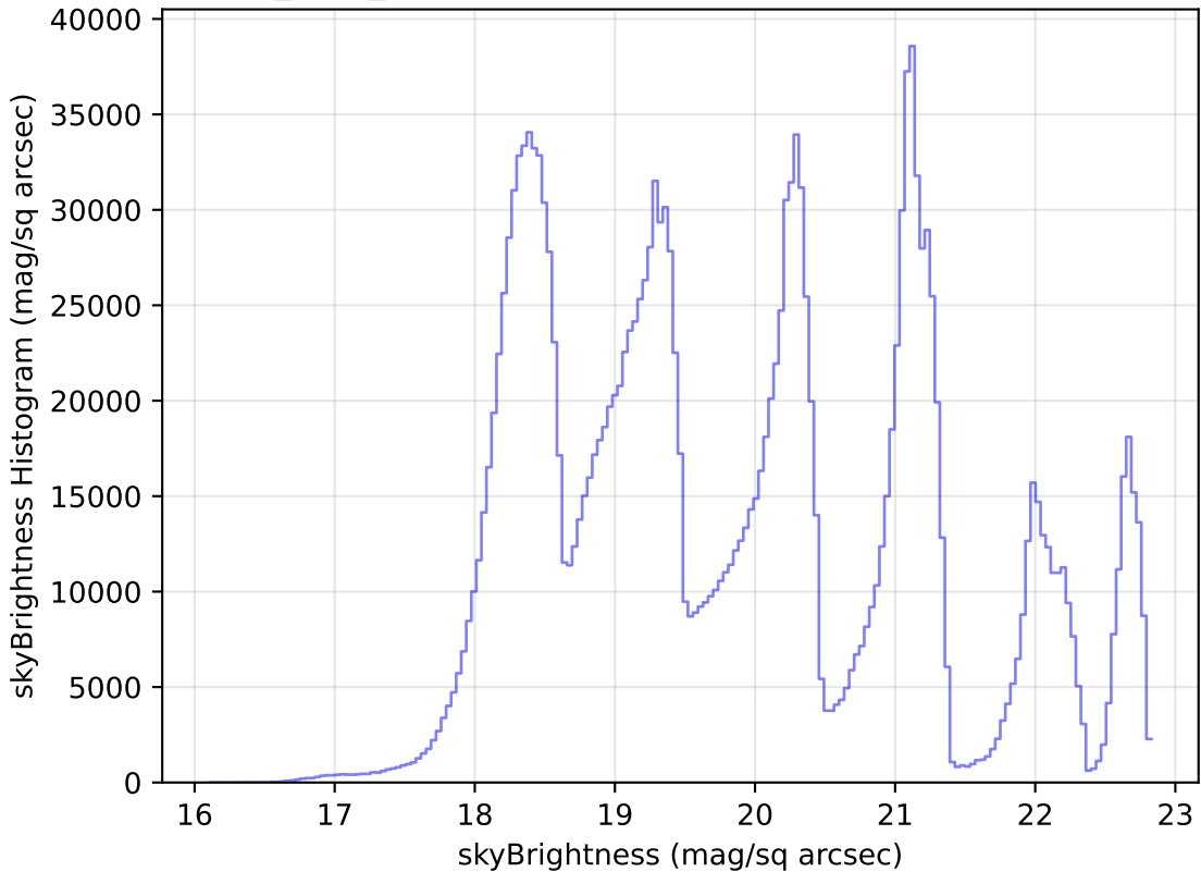
baseline_v3.2_10yrs All sky all bands: skyBrightness Histogram
