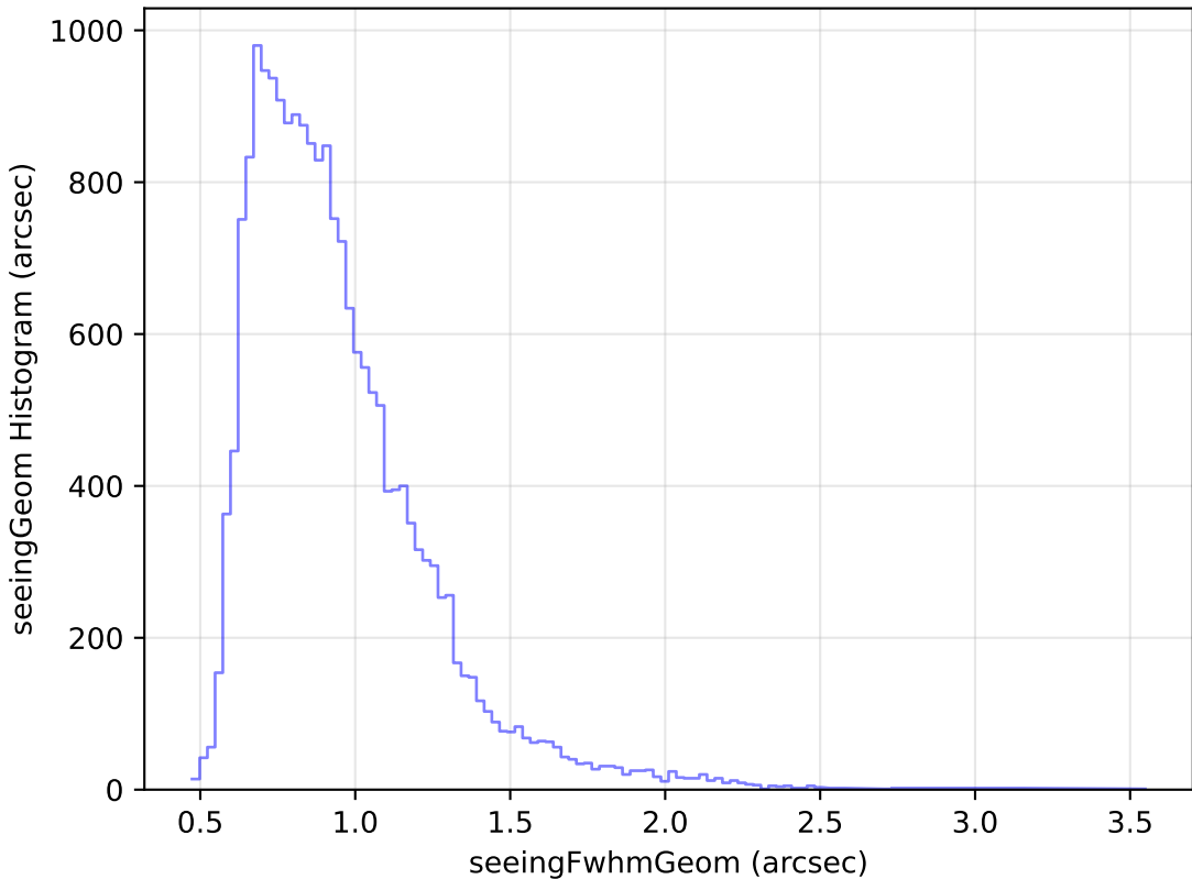
baseline_v3.2_10yrs Yr 1 g band: seeingGeom Histogram
