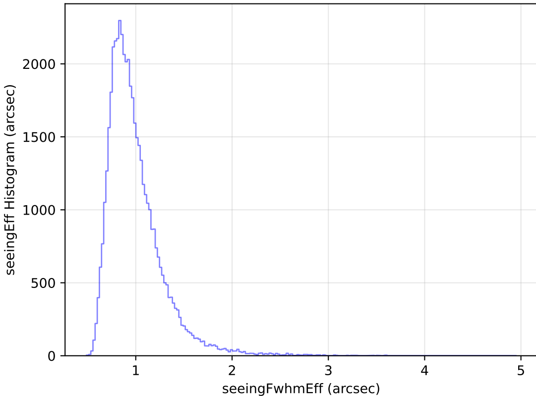
baseline_v3.2_10yrs Yr 1 z band: seeingEff Histogram
