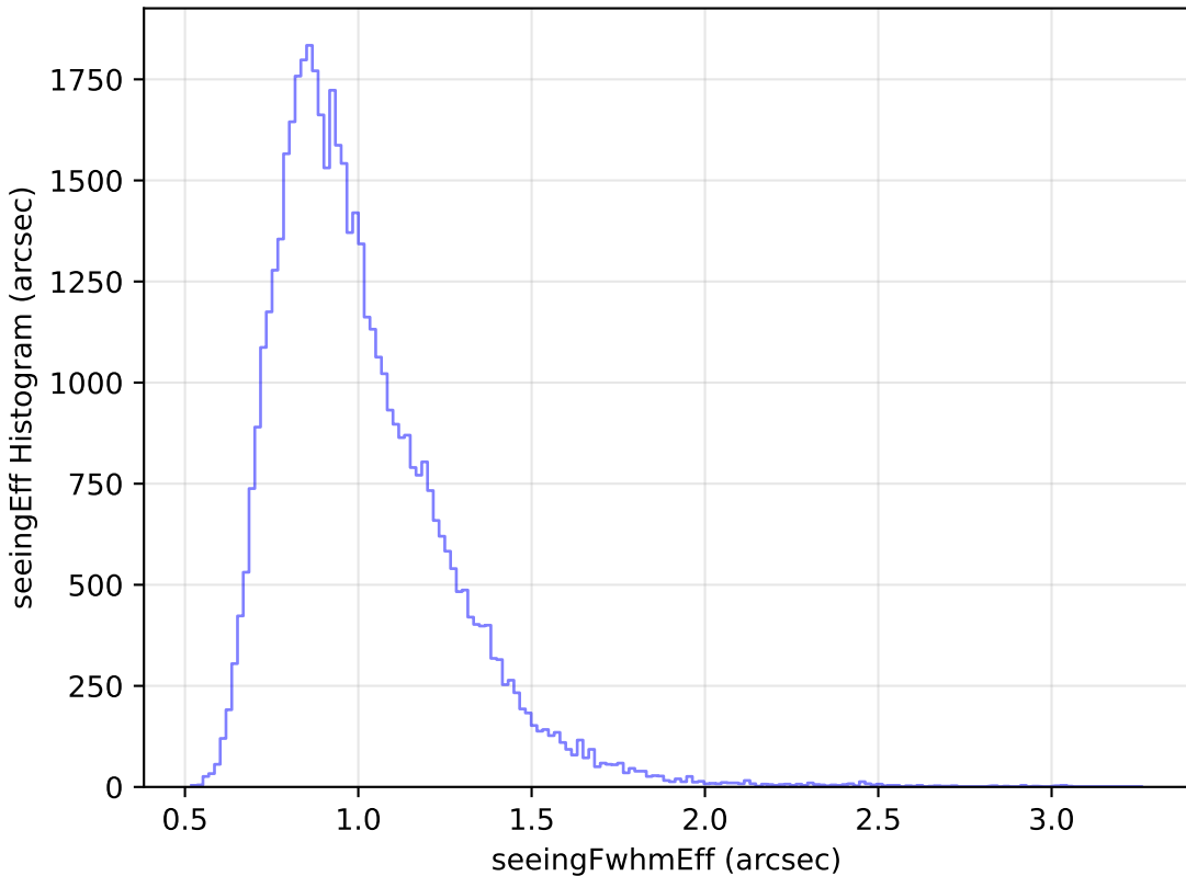
baseline_v3.2_10yrs Yr 1 y band: seeingEff Histogram
