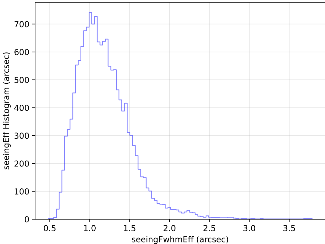
baseline_v3.2_10yrs Yr 1 u band: seeingEff Histogram
