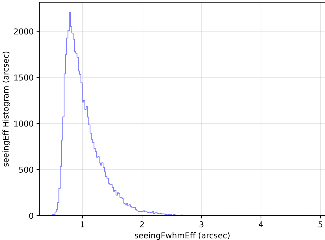
baseline_v3.2_10yrs Yr 1 r band: seeingEff Histogram
