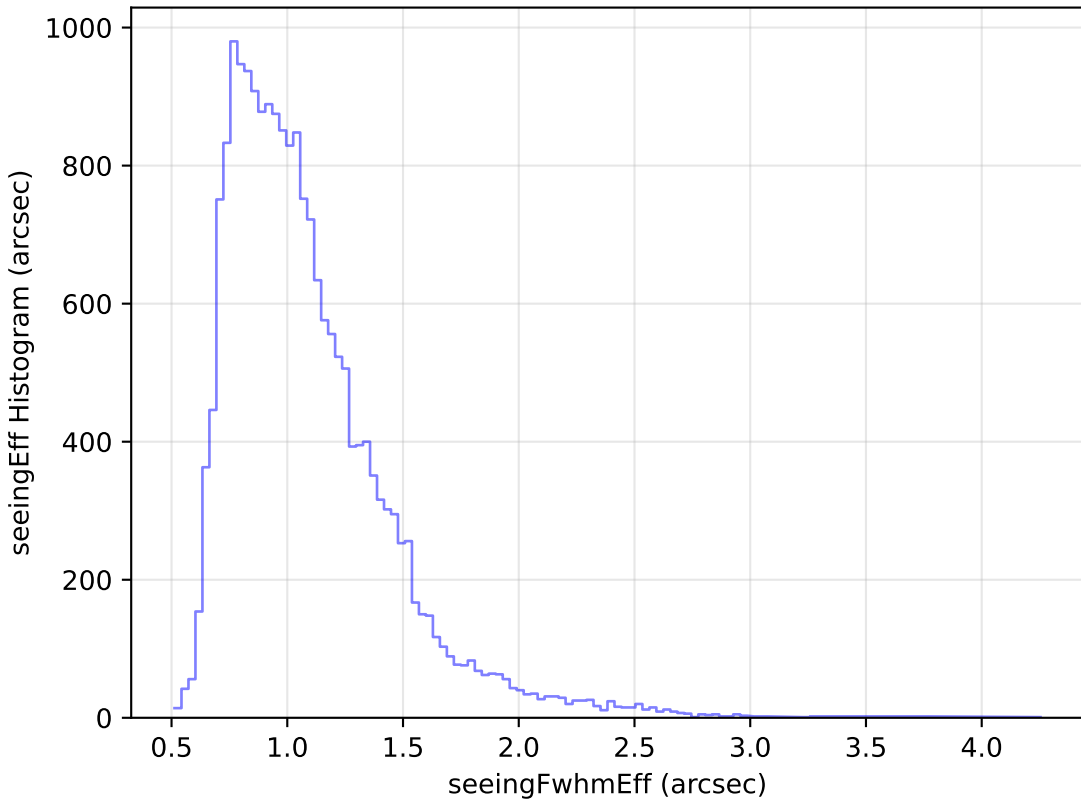
baseline_v3.2_10yrs Yr 1 g band: seeingEff Histogram
