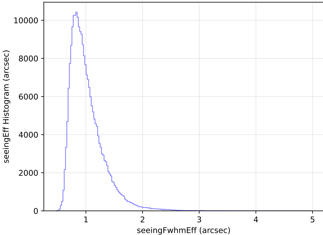
baseline_v3.2_10yrs Yr 1 all bands: seeingEff Histogram
