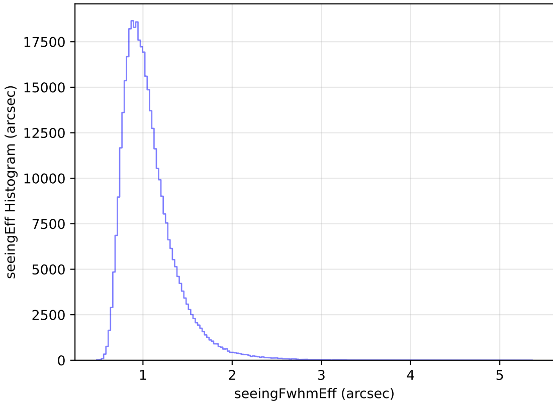
baseline_v3.2_10yrs WFD y band: seeingEff Histogram
