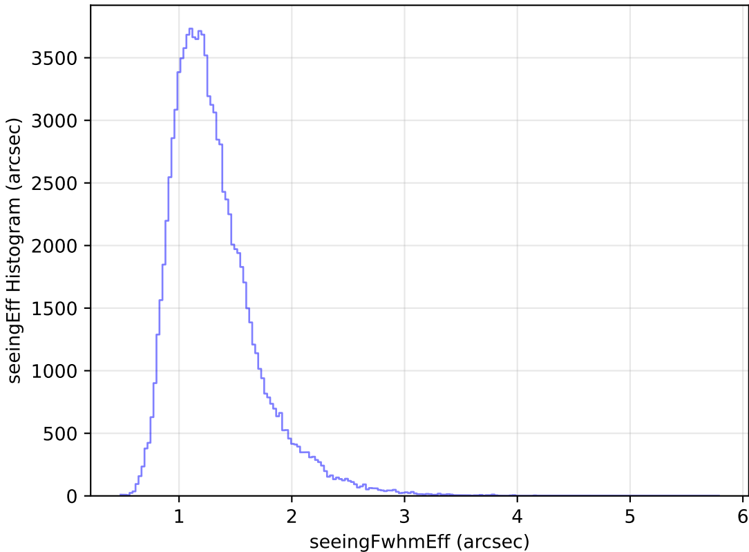
baseline_v3.2_10yrs WFD u band: seeingEff Histogram
