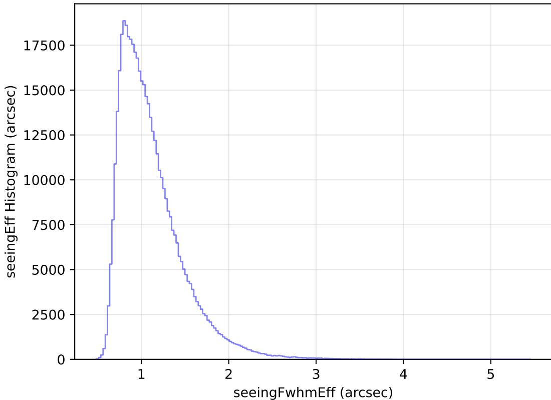
baseline_v3.2_10yrs WFD r band: seeingEff Histogram
