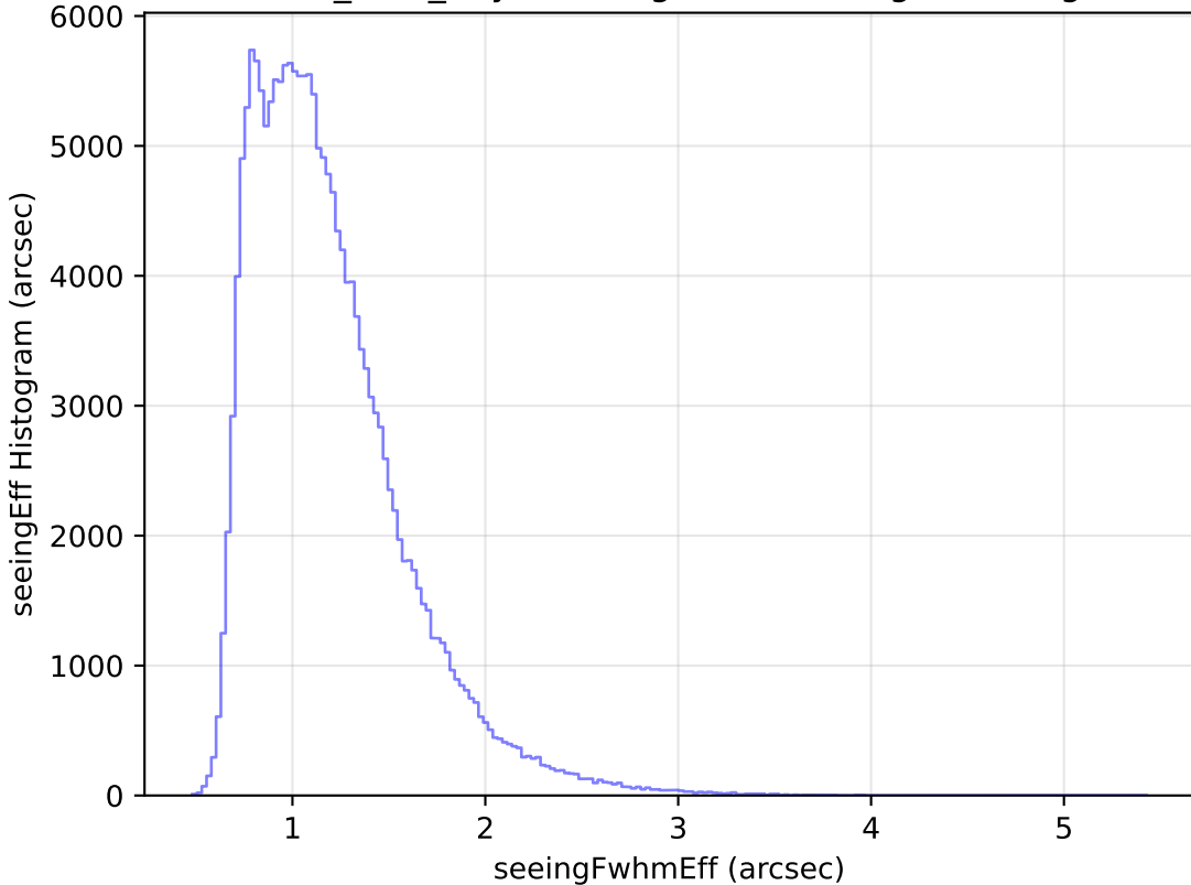
baseline_v3.2_10yrs WFD g band: seeingEff Histogram
