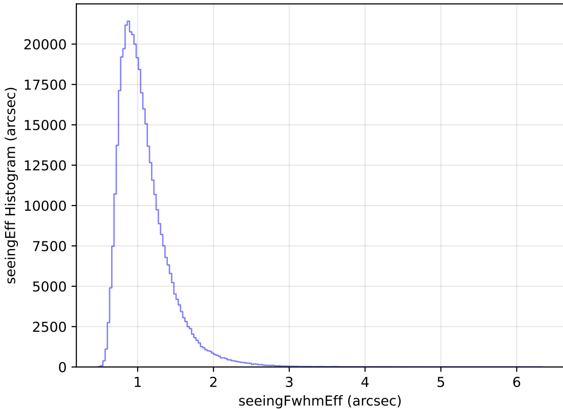
baseline_v3.2_10yrs All sky z band: seeingEff Histogram
