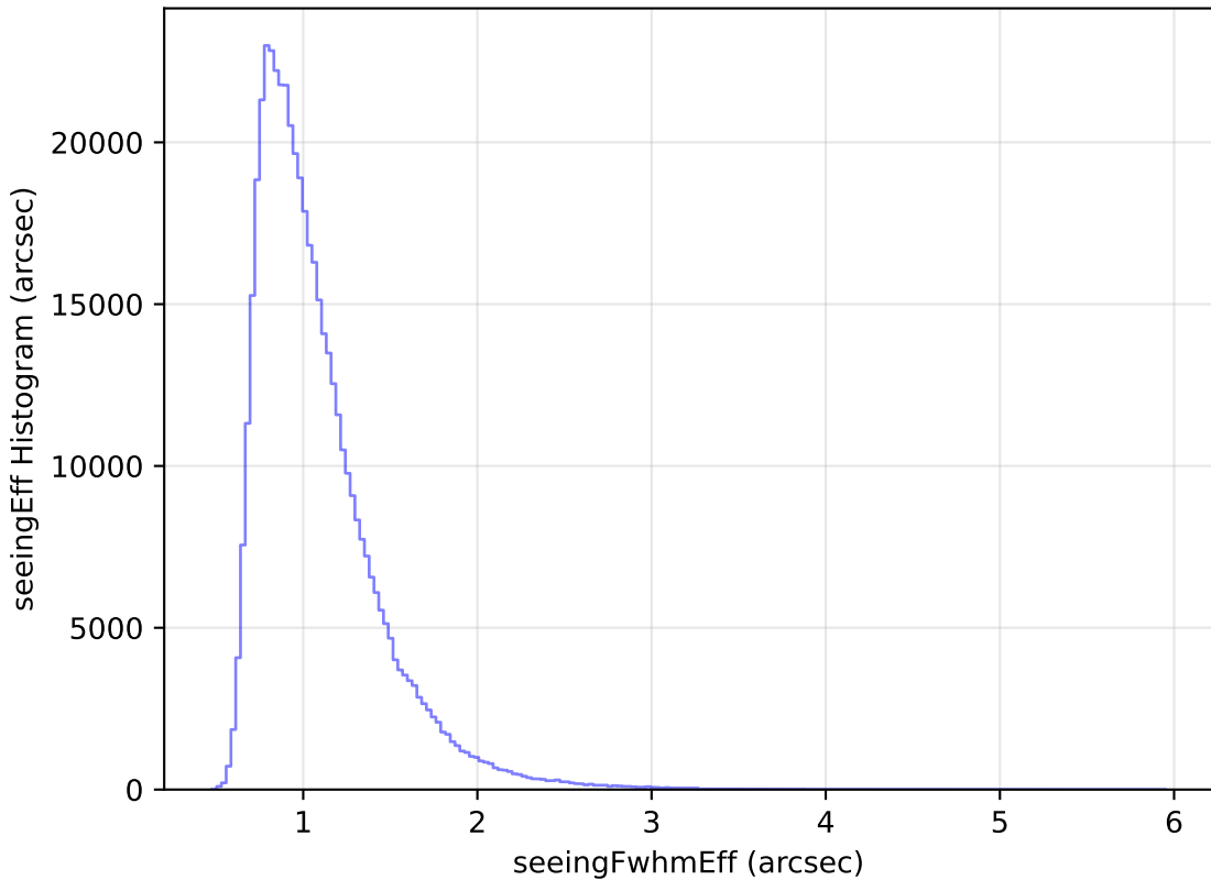
baseline_v3.2_10yrs All sky i band: seeingEff Histogram
