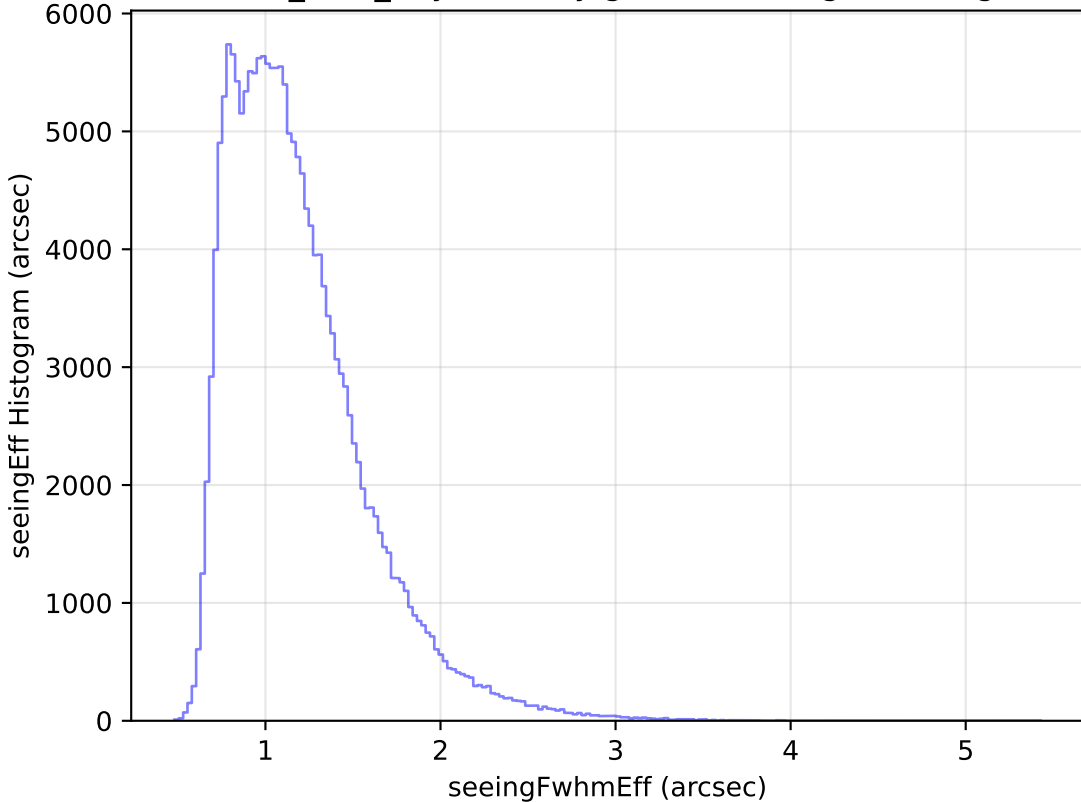
baseline_v3.2_10yrs All sky g band: seeingEff Histogram
