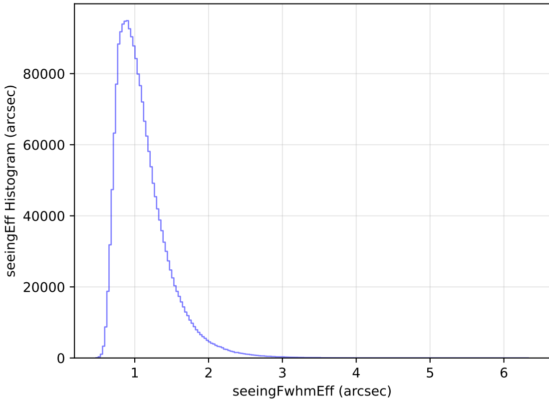
baseline_v3.2_10yrs All sky all bands: seeingEff Histogram
