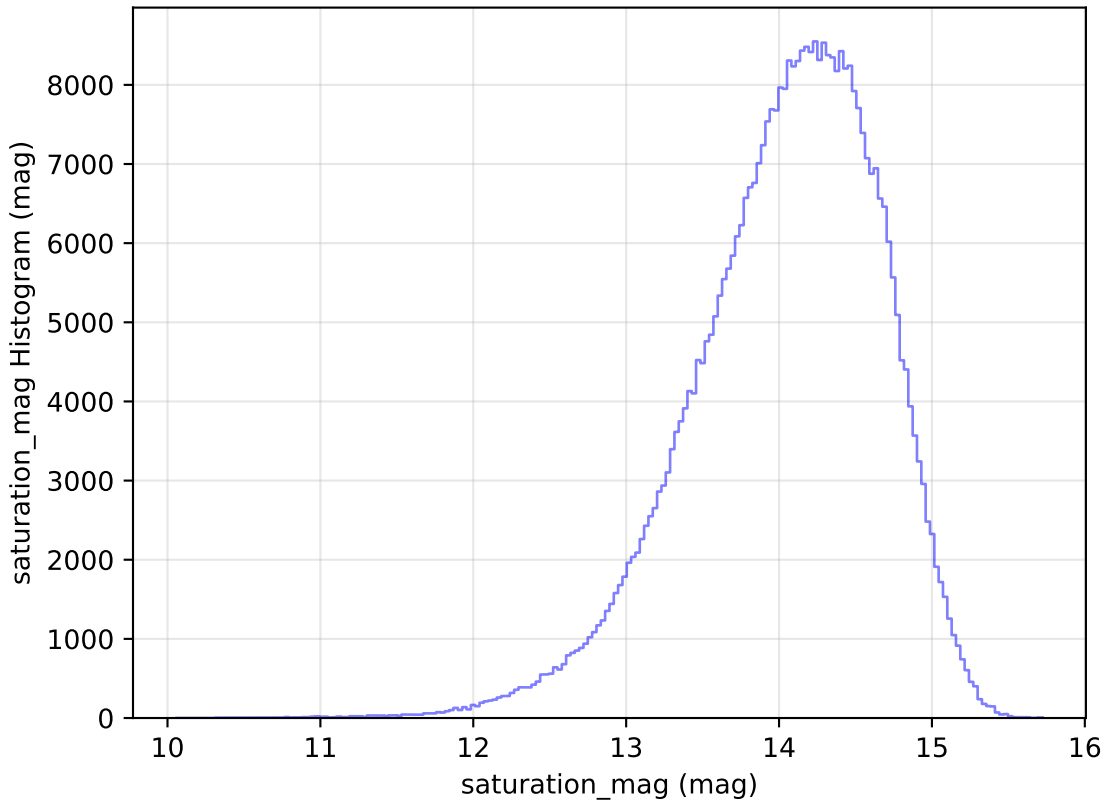
baseline_v3.2_10yrs WFD z band: saturation_mag Histogram
