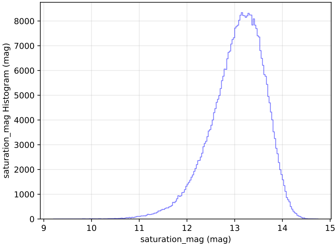
baseline_v3.2_10yrs WFD y band: saturation_mag Histogram
