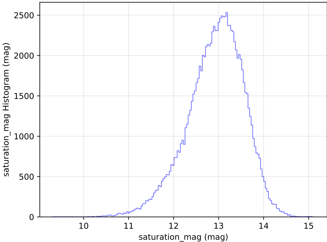
baseline_v3.2_10yrs WFD u band: saturation_mag Histogram
