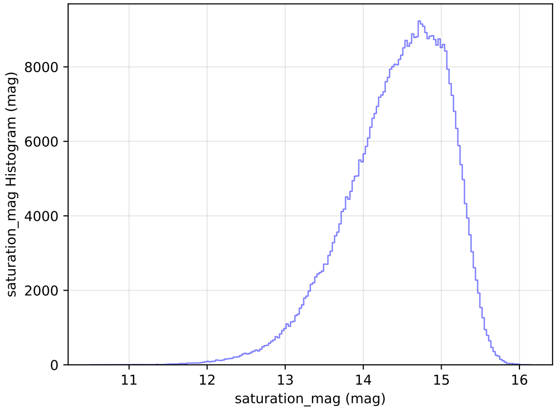
baseline_v3.2_10yrs WFD i band: saturation_mag Histogram
