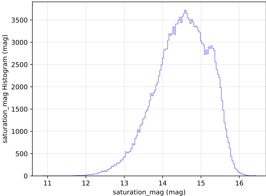
baseline_v3.2_10yrs WFD g band: saturation_mag Histogram
