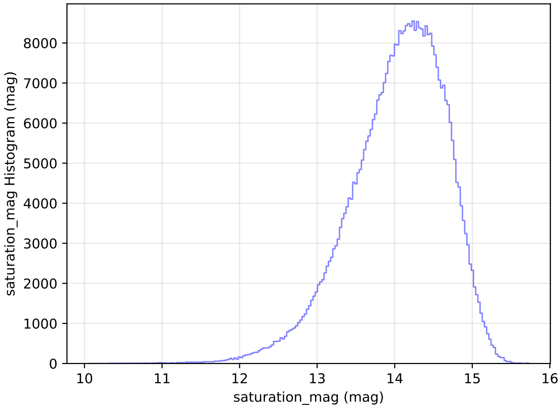
baseline_v3.2_10yrs All sky z band: saturation_mag Histogram
