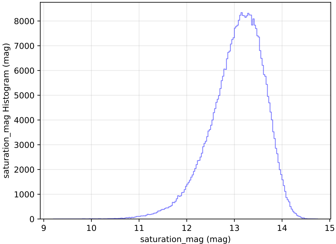
baseline_v3.2_10yrs All sky y band: saturation_mag Histogram
