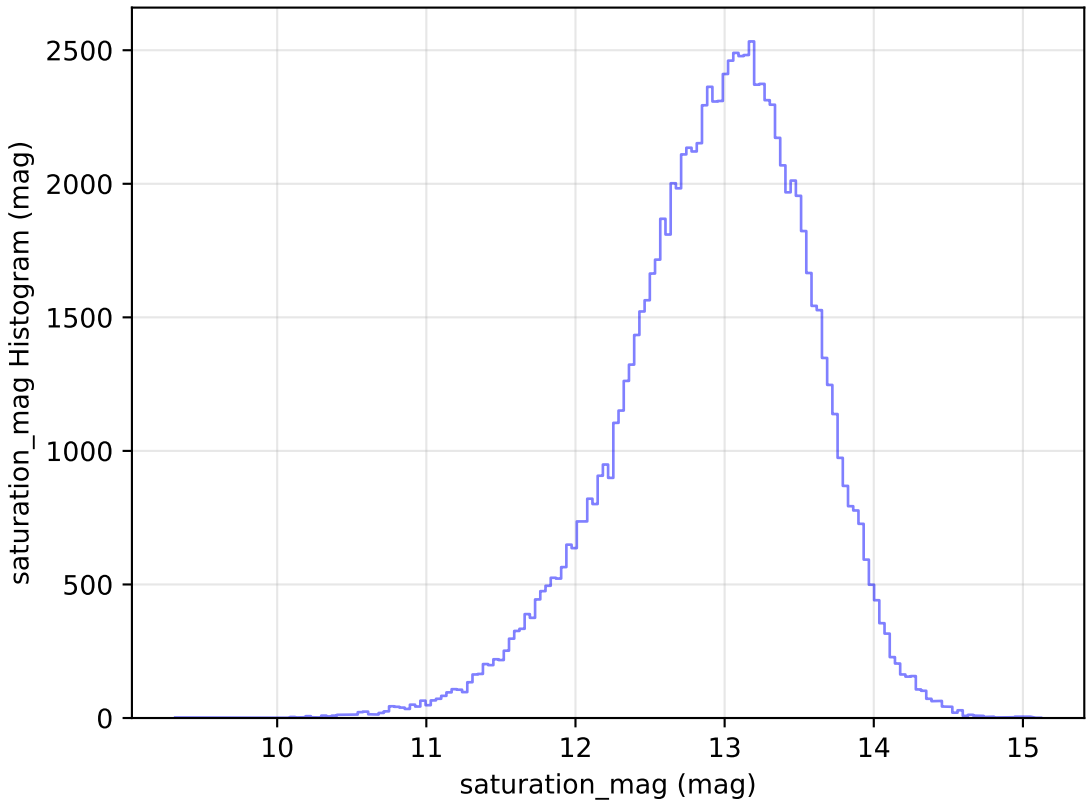
baseline_v3.2_10yrs All sky u band: saturation_mag Histogram
