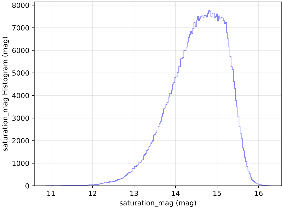
baseline_v3.2_10yrs All sky r band: saturation_mag Histogram
