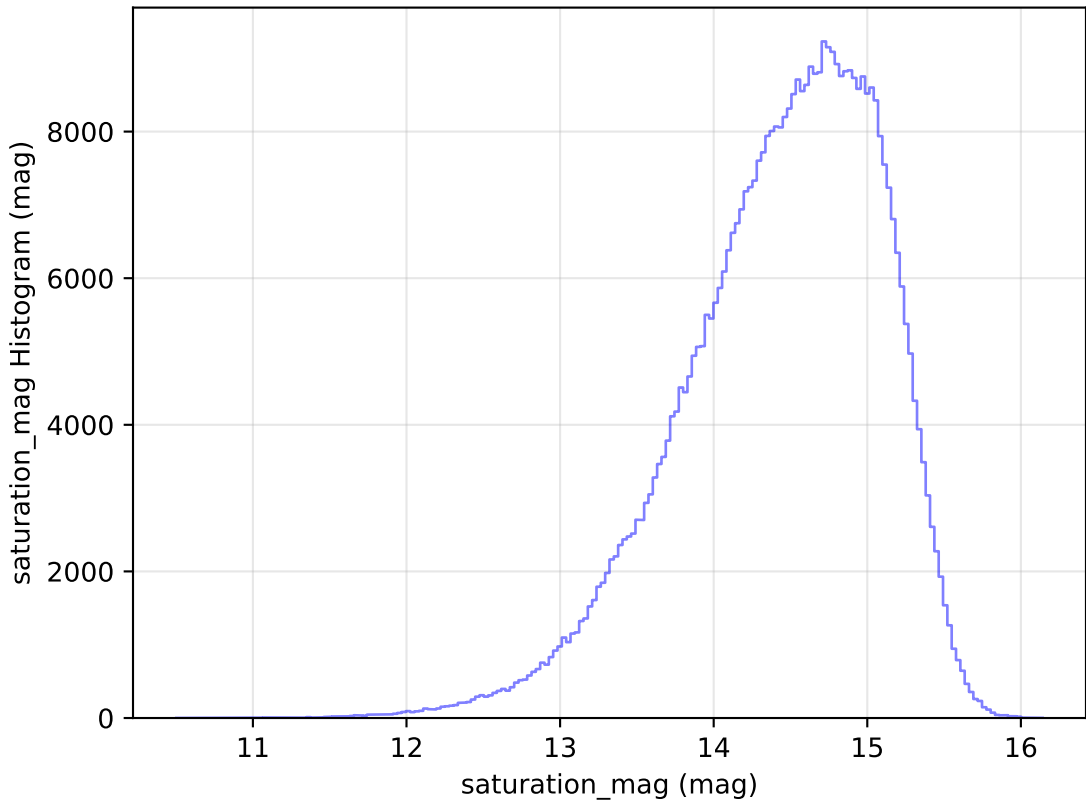
baseline_v3.2_10yrs All sky i band: saturation_mag Histogram
