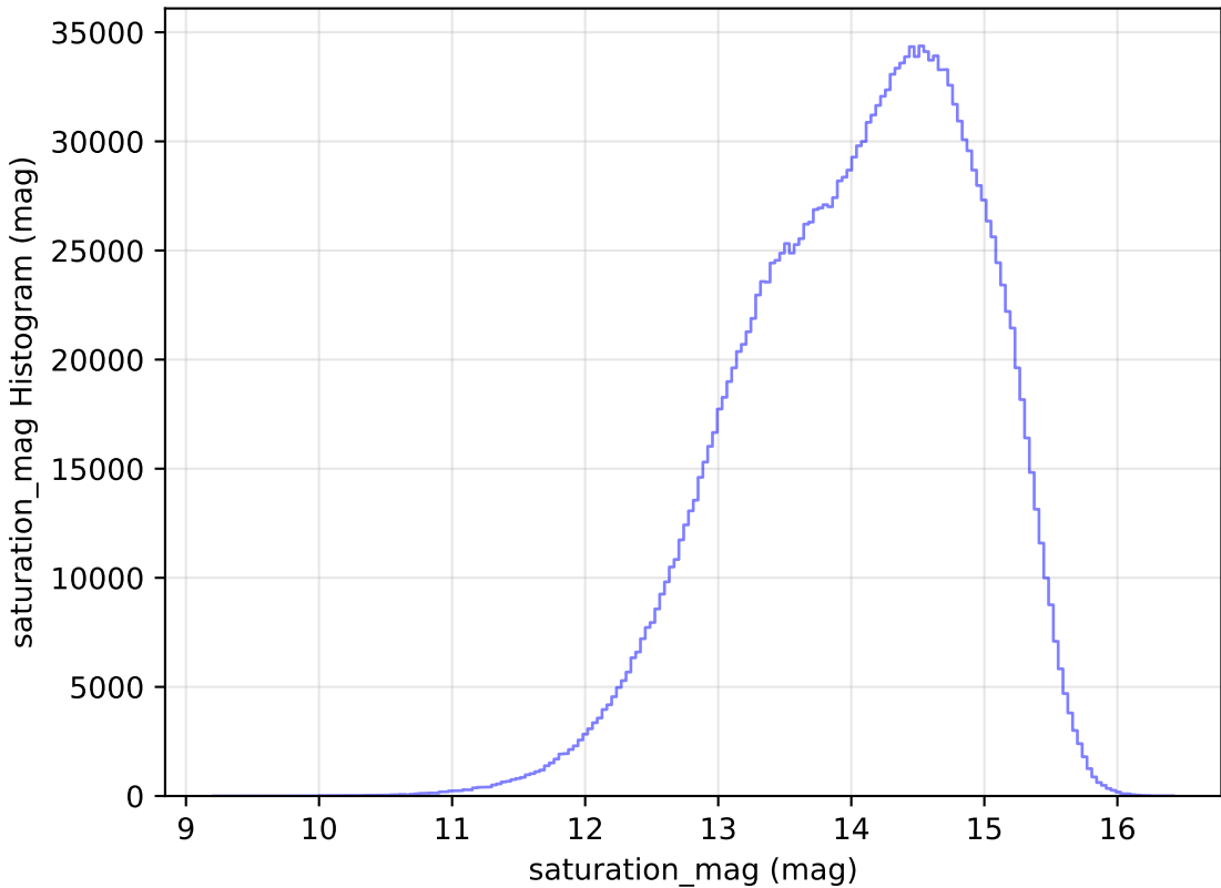
baseline_v3.2_10yrs All sky all bands: saturation_mag Histogram
