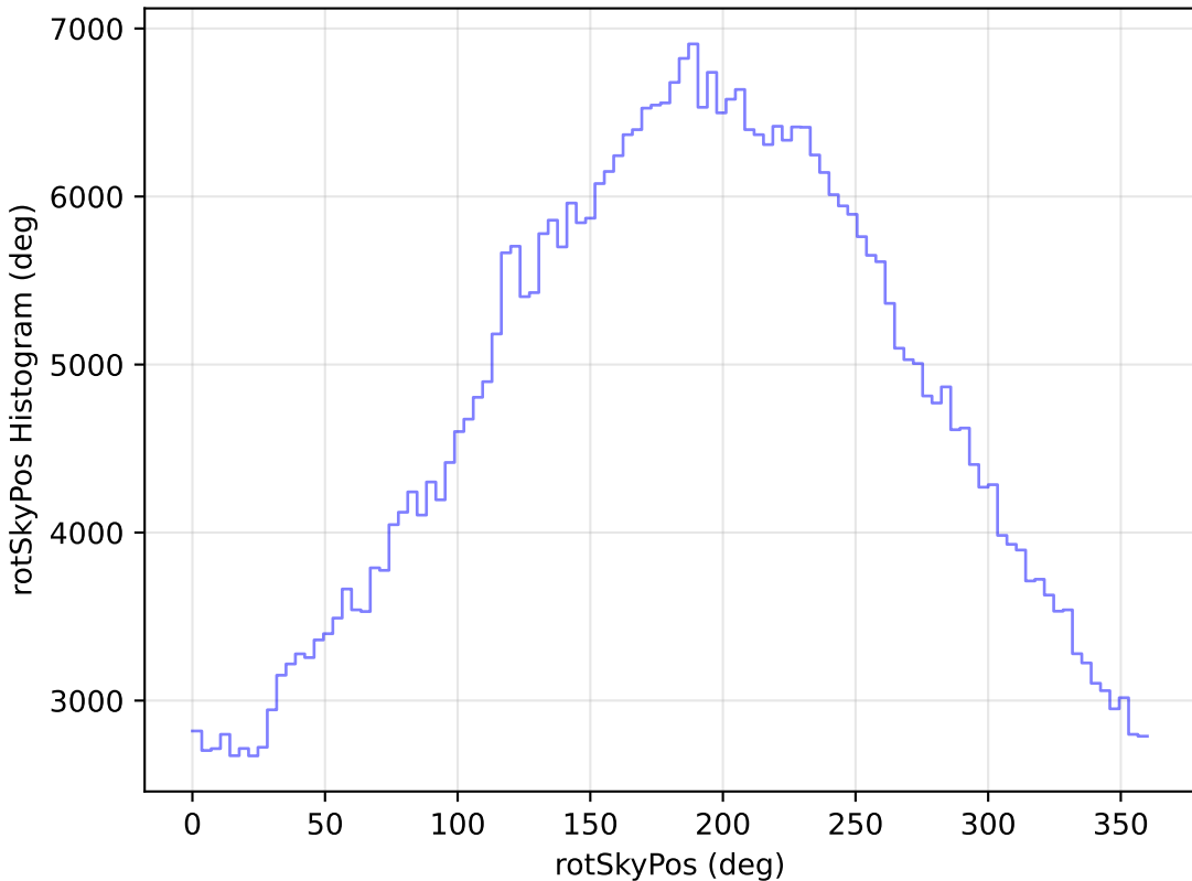
baseline_v3.2_10yrs WFD r band: rotSkyPos Histogram
