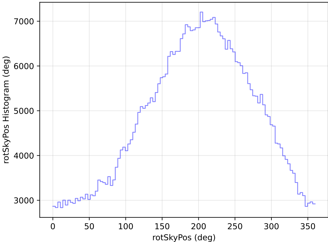
baseline_v3.2_10yrs WFD i band: rotSkyPos Histogram
