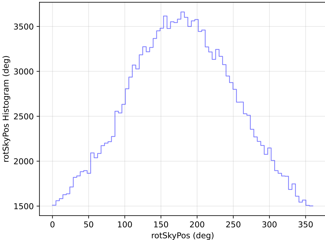
baseline_v3.2_10yrs WFD g band: rotSkyPos Histogram
