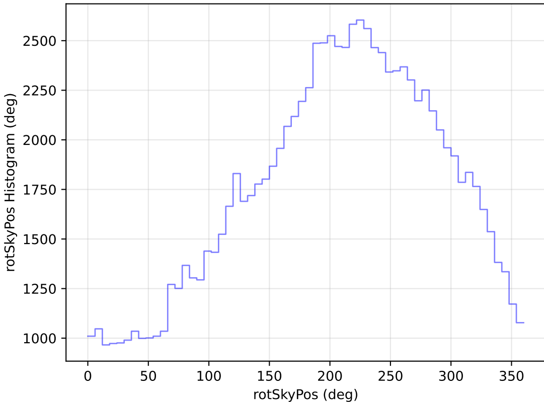
baseline_v3.2_10yrs All sky u band: rotSkyPos Histogram
