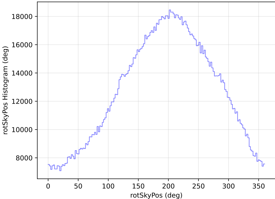
baseline_v3.2_10yrs All sky all bands: rotSkyPos Histogram
