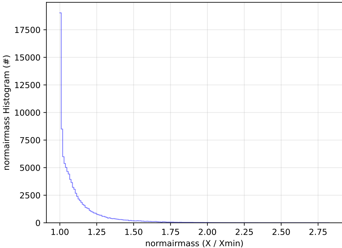
baseline_v3.2_10yrs WFD u band: normairmass Histogram
