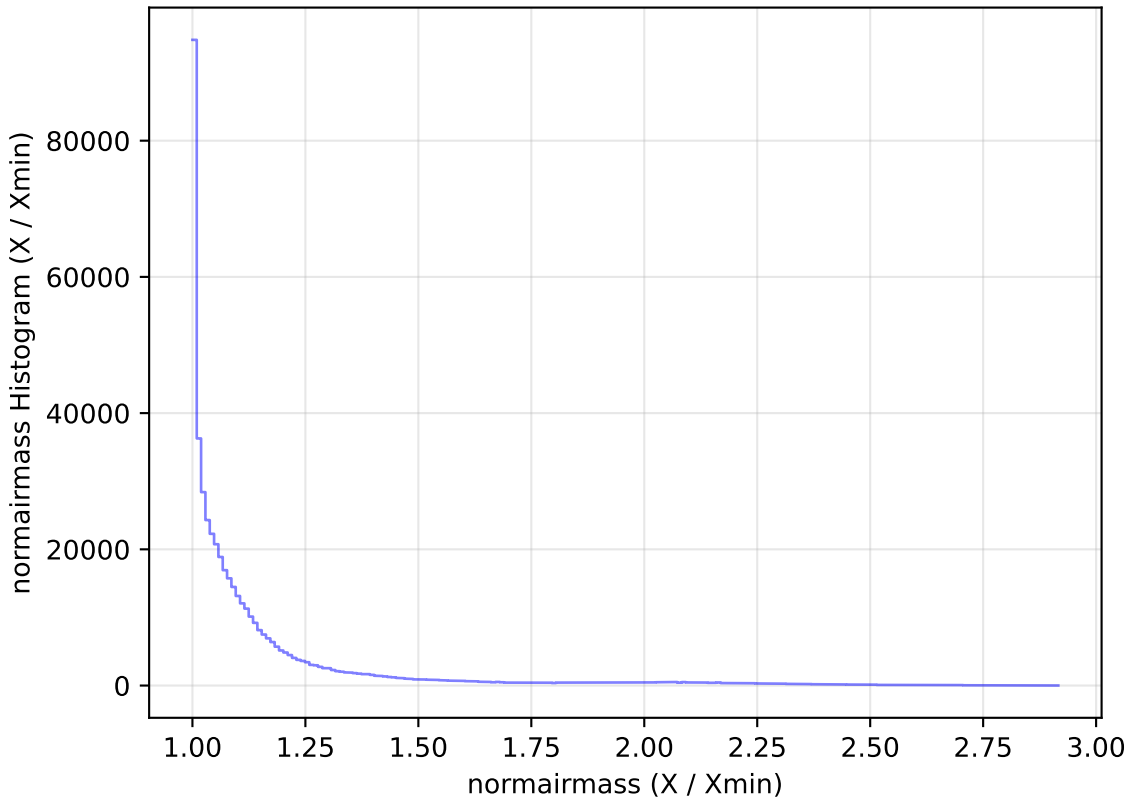
baseline_v3.2_10yrs WFD i band: normairmass Histogram
