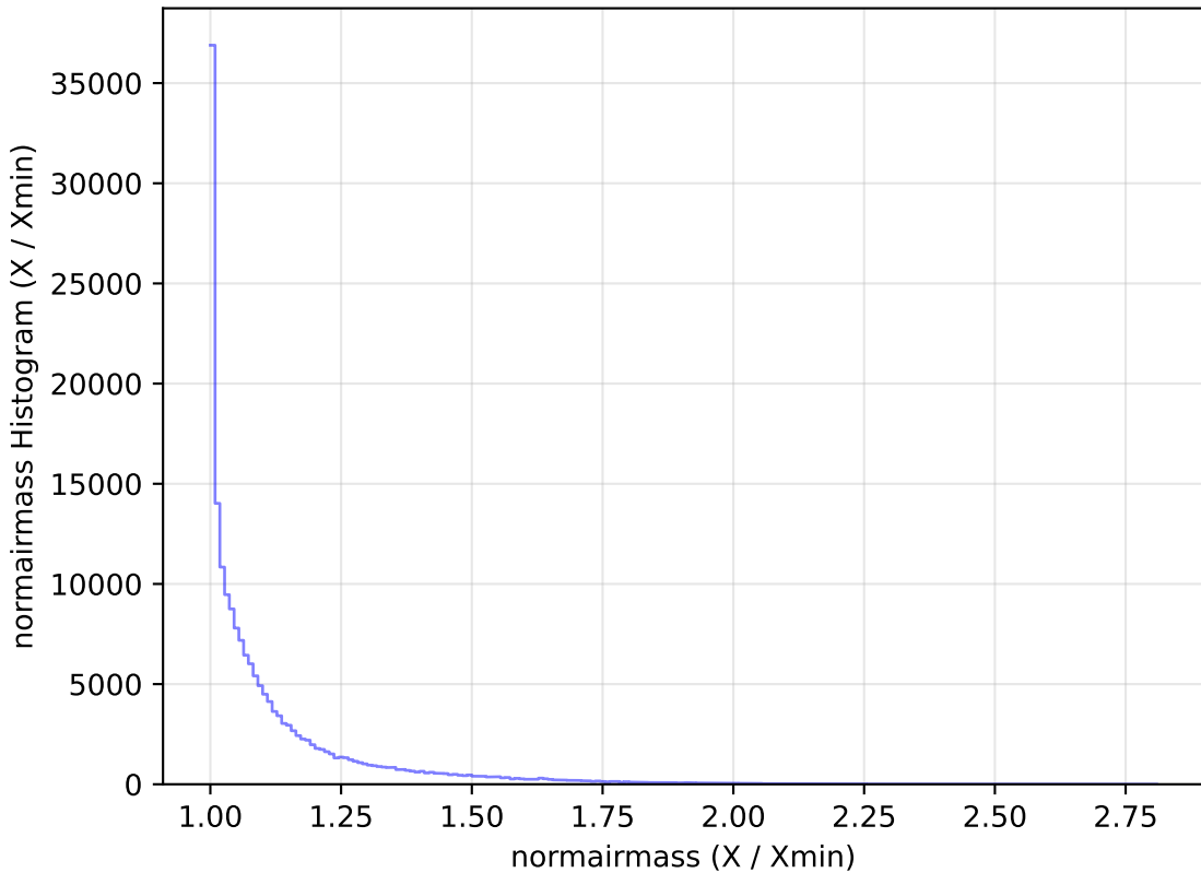
baseline_v3.2_10yrs WFD g band: normairmass Histogram
