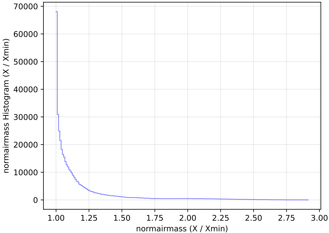
baseline_v3.2_10yrs All sky z band: normairmass Histogram
