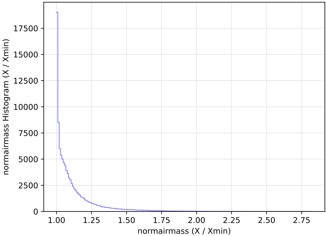
baseline_v3.2_10yrs All sky u band: normairmass Histogram
