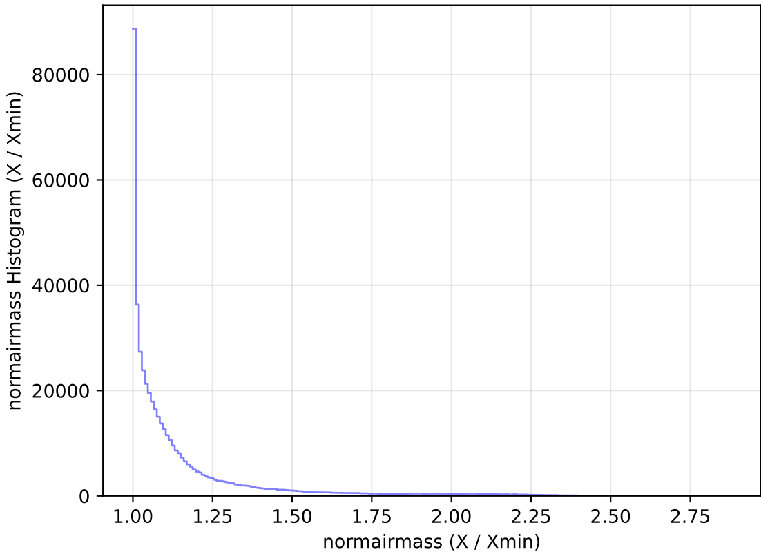
baseline_v3.2_10yrs All sky r band: normairmass Histogram
