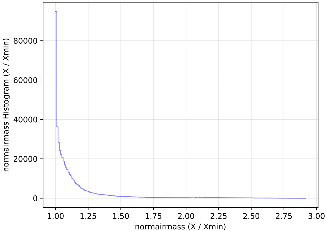
baseline_v3.2_10yrs All sky i band: normairmass Histogram
