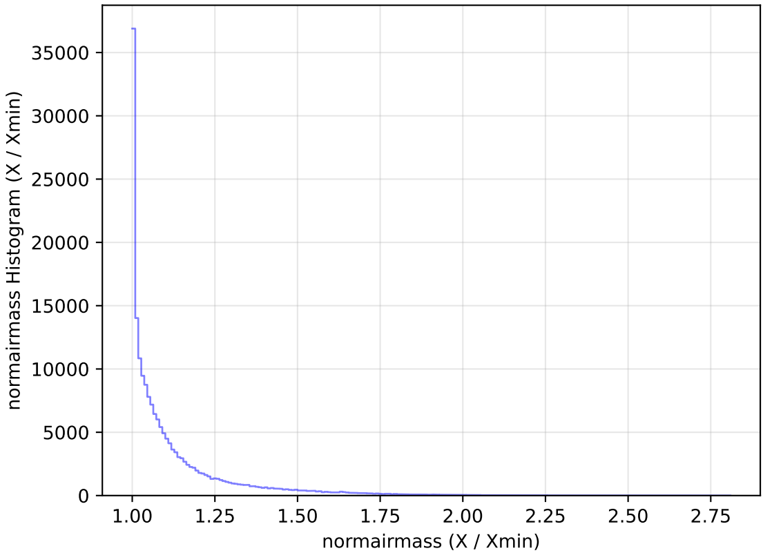
baseline_v3.2_10yrs All sky g band: normairmass Histogram
