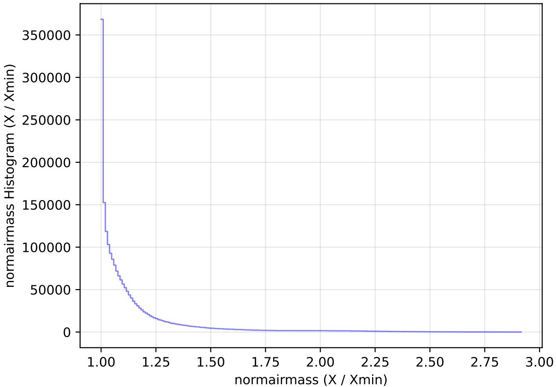
baseline_v3.2_10yrs All sky all bands: normairmass Histogram
