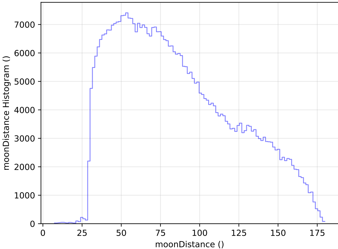
baseline_v3.2_10yrs WFD z band: moonDistance Histogram
