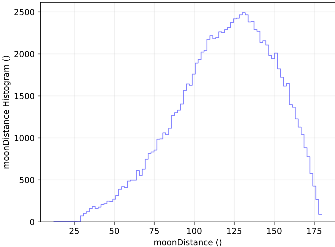
baseline_v3.2_10yrs WFD u band: moonDistance Histogram
