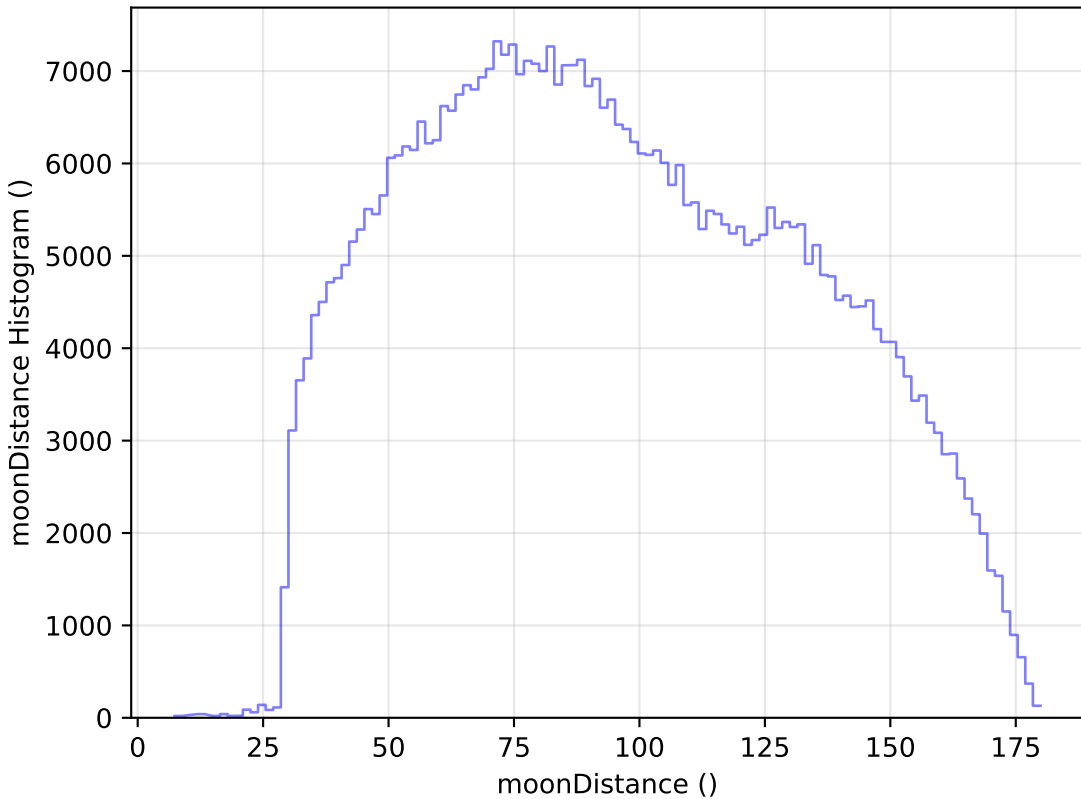
baseline_v3.2_10yrs WFD i band: moonDistance Histogram
