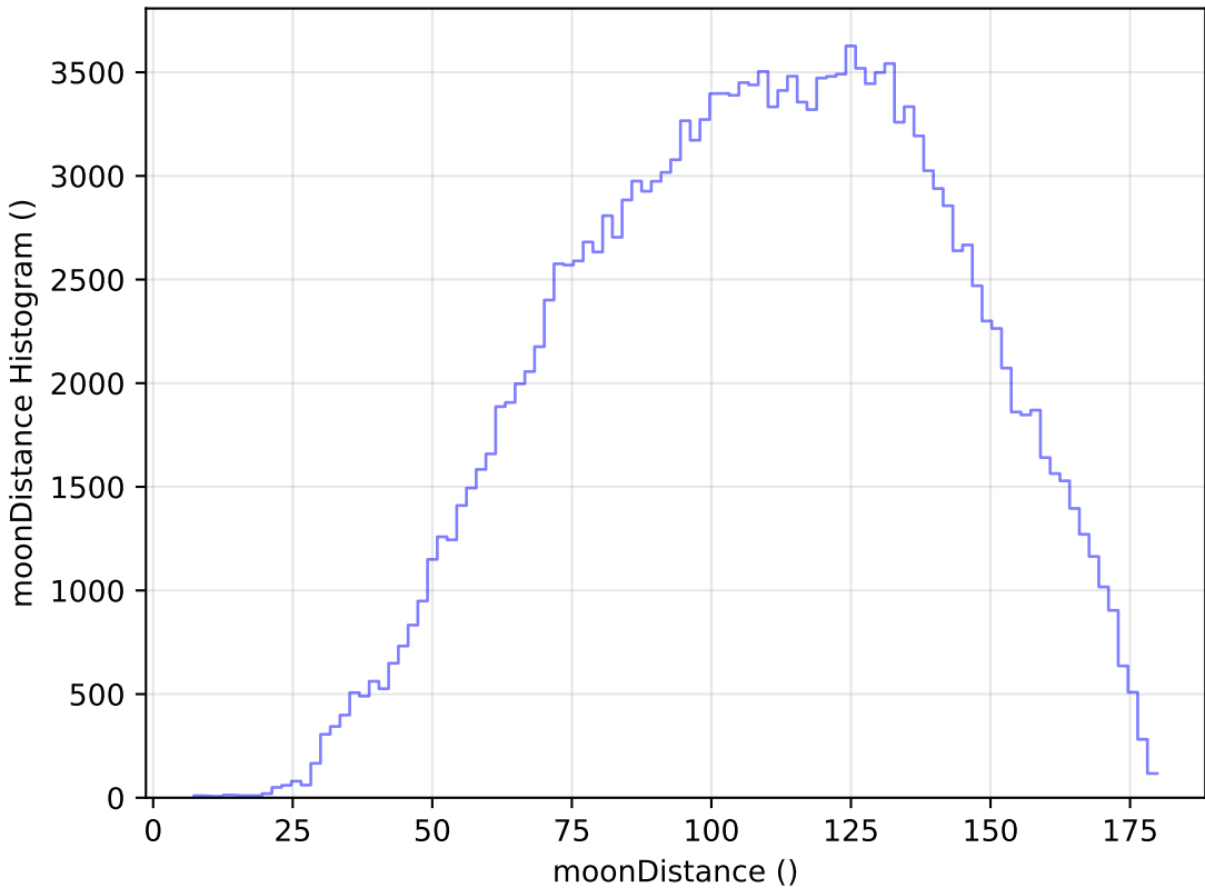
baseline_v3.2_10yrs WFD g band: moonDistance Histogram
